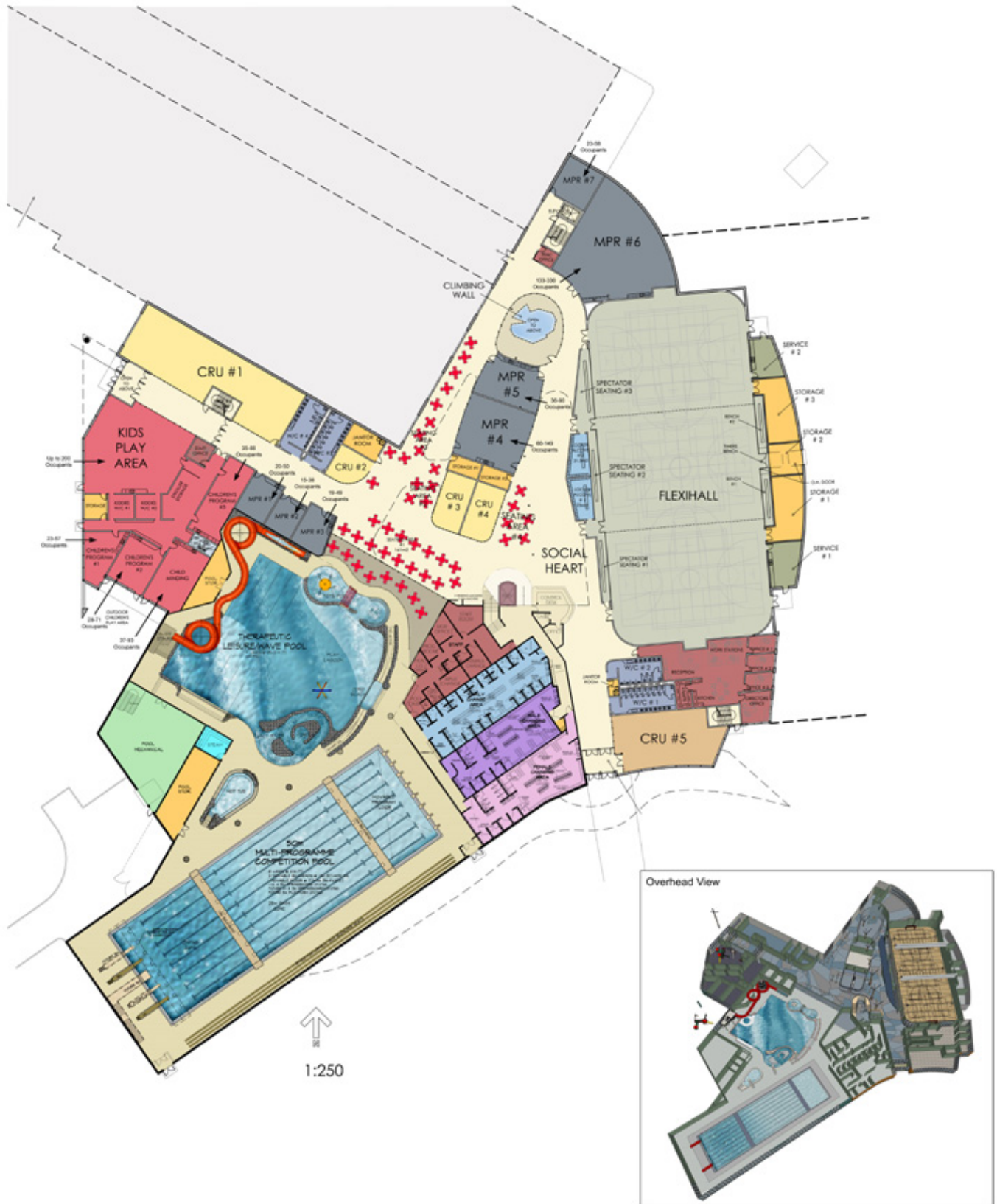
Floor Plan
